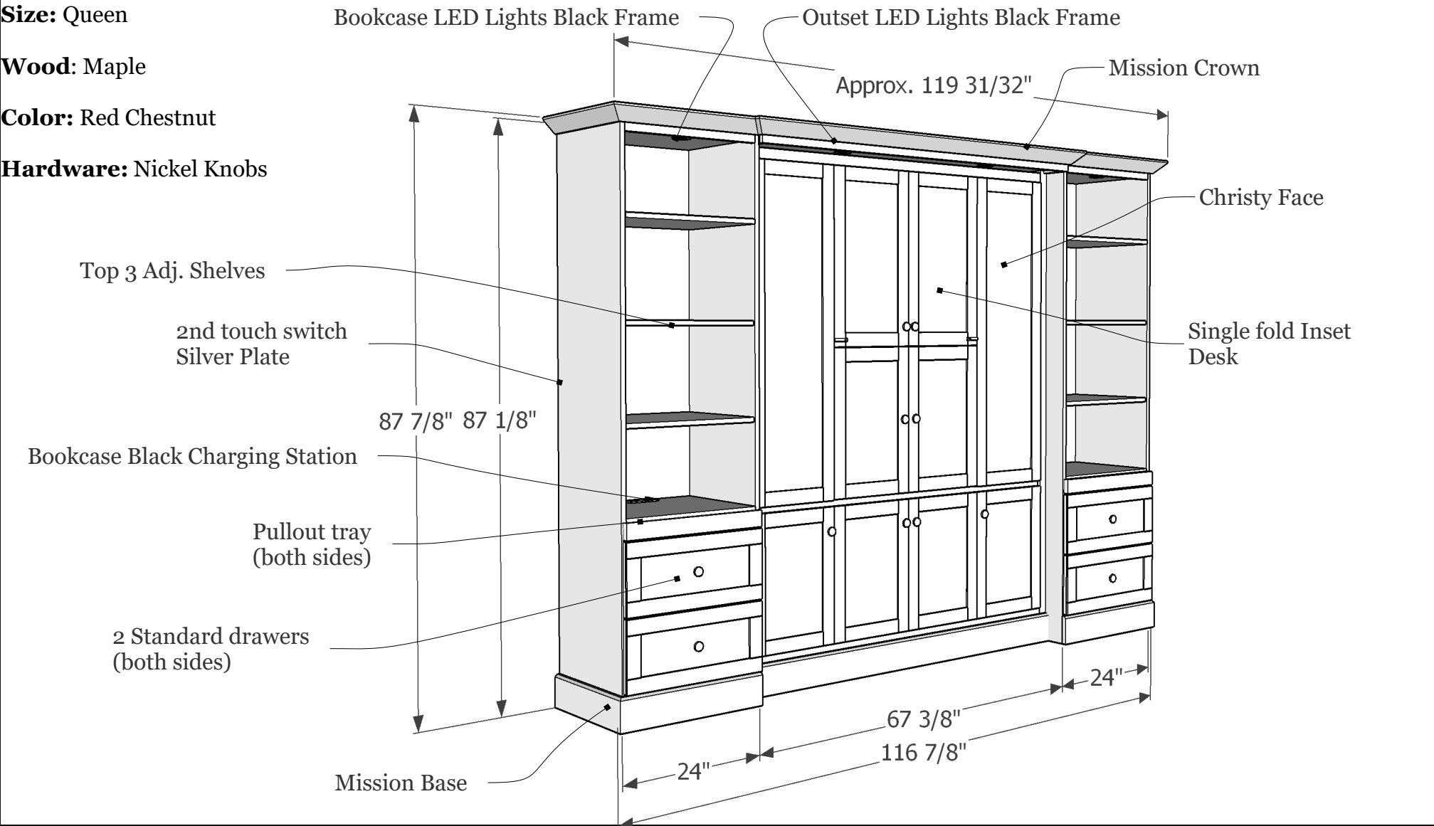
Main Drawing with Measurements
