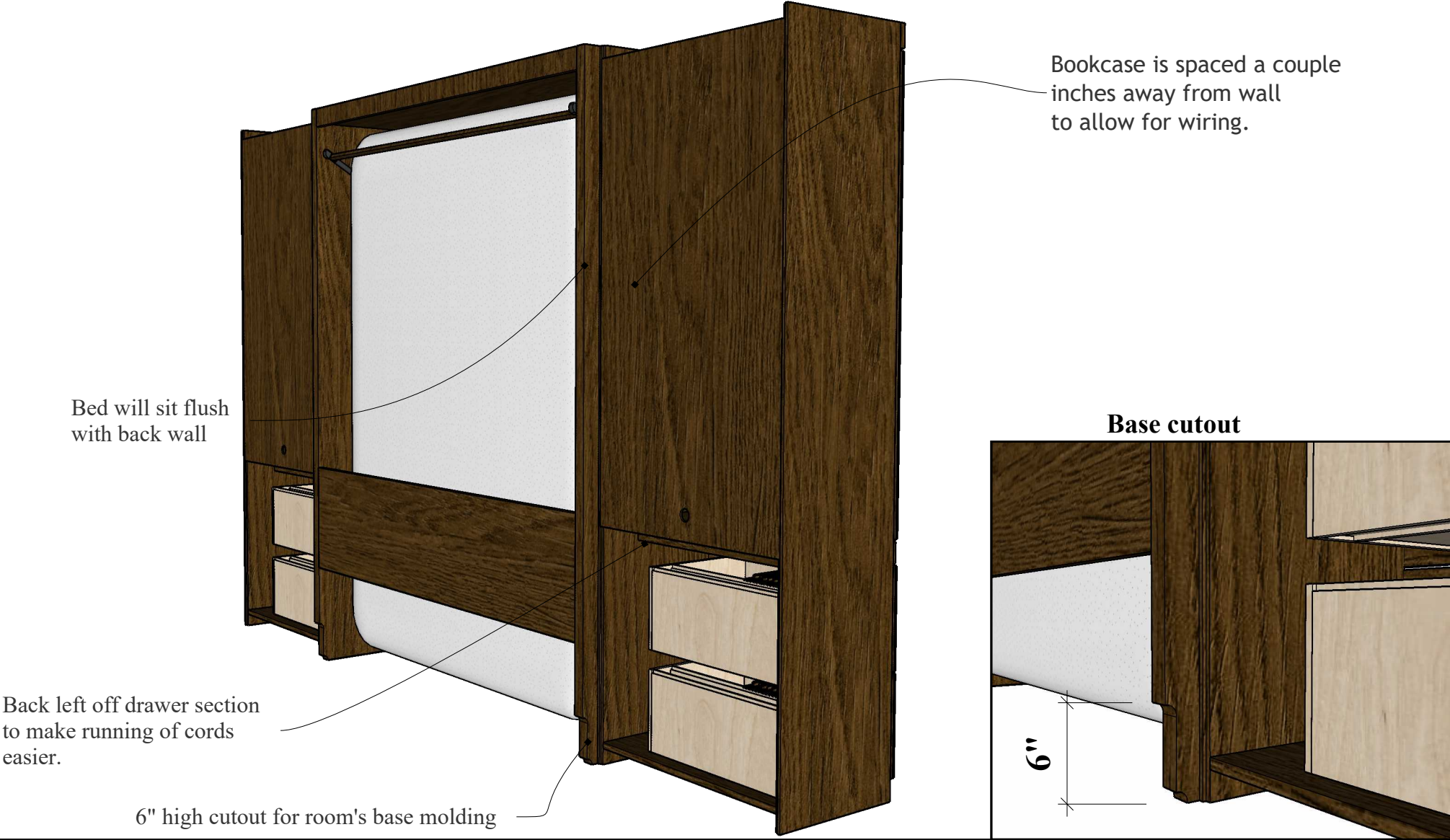
Base Molding Cutout
