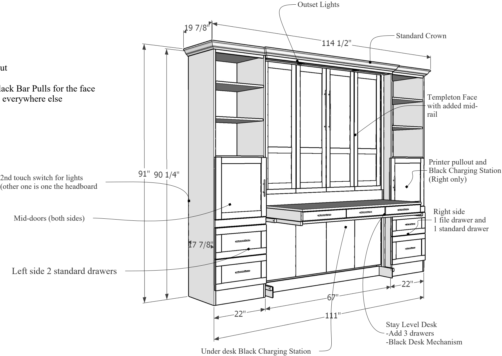
Main Drawing with Measurements
