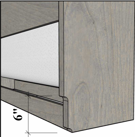
Base cutout
