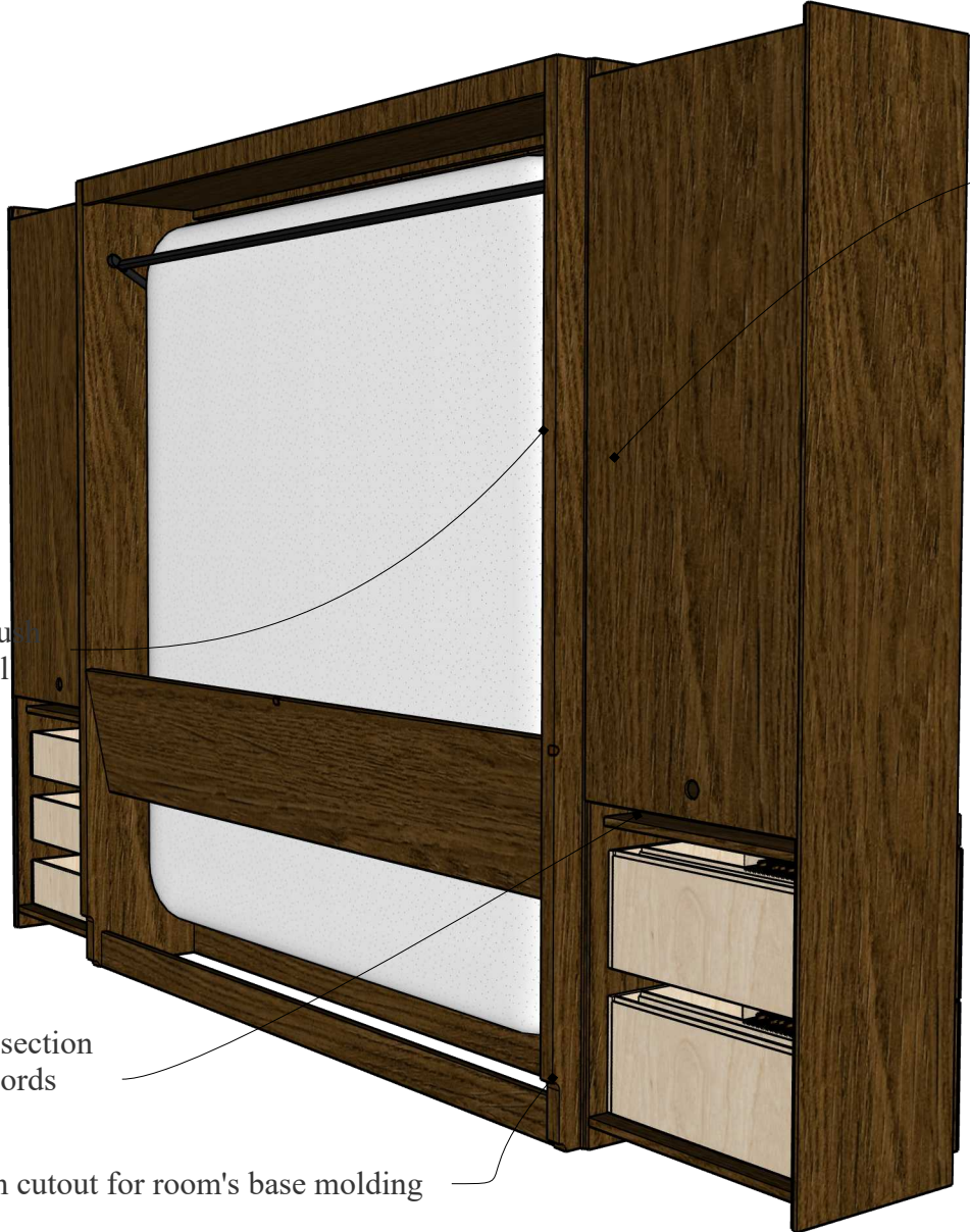
Base Molding Cutout
