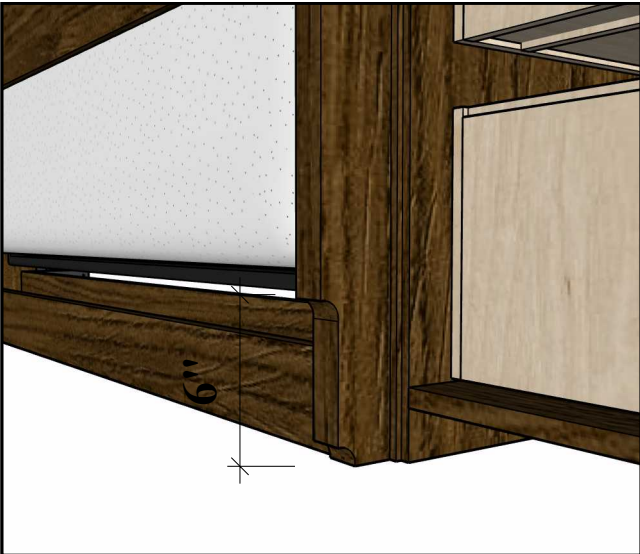
Base cutout
