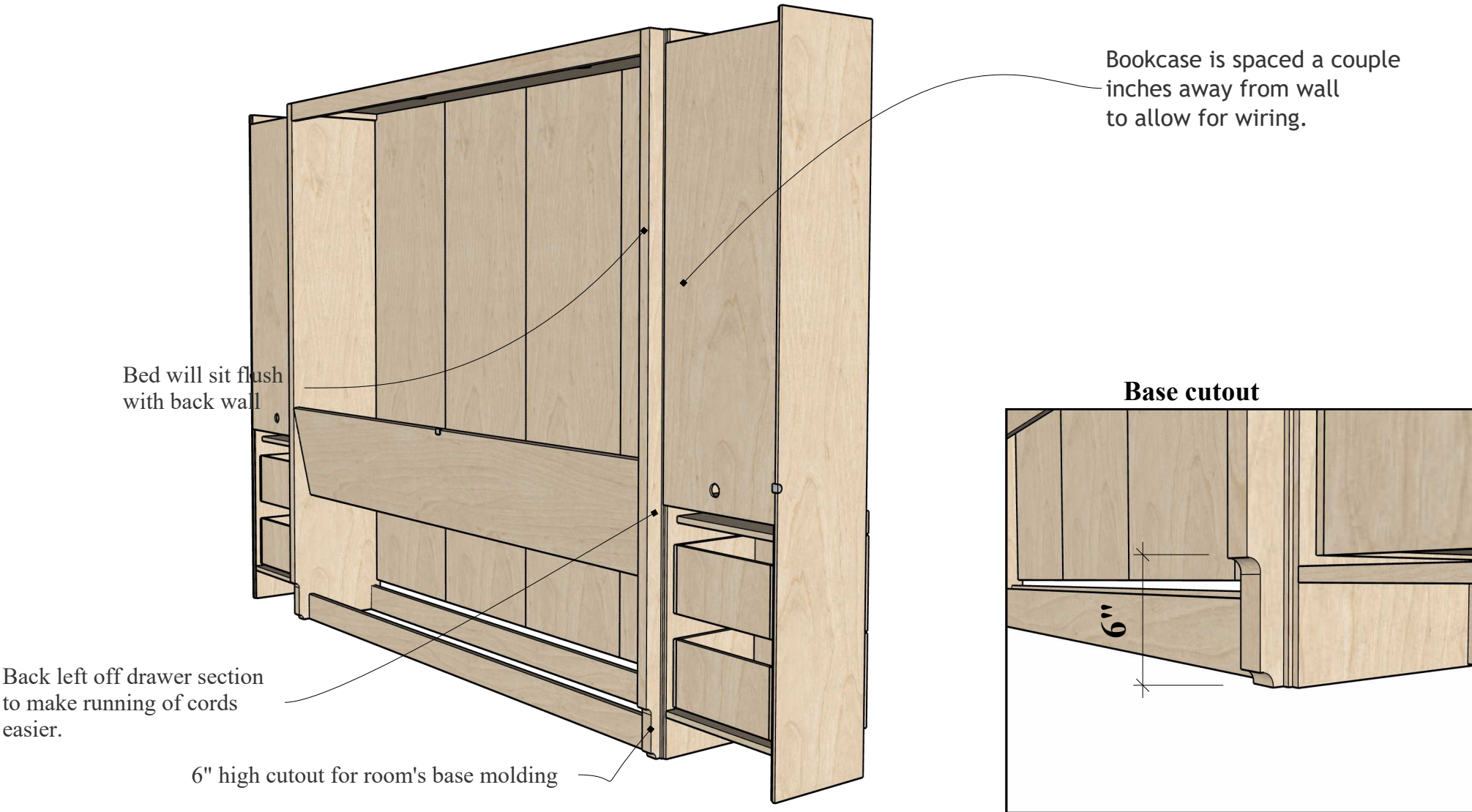
Base Molding Cutout
