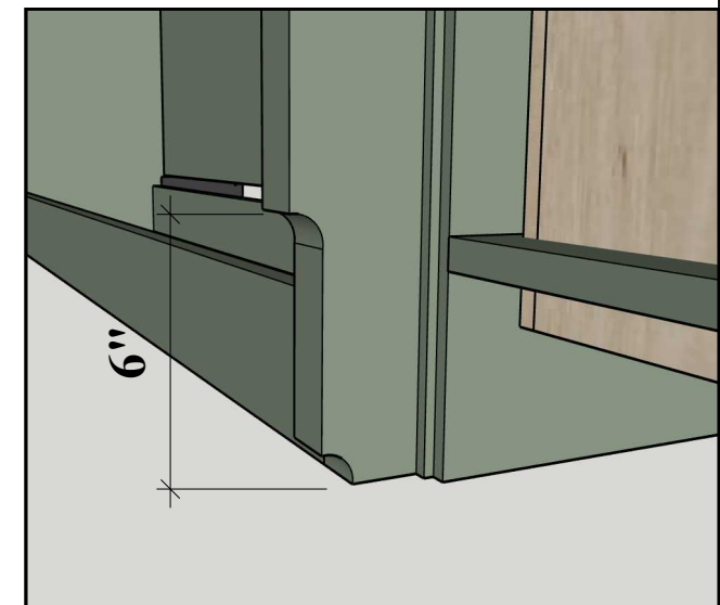
Base cutout
